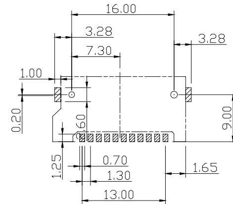
Recommended PCB Layout (PCB TOLERANCE±0.05)
